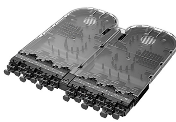
Кассета EHD 24 port LC field term splice cassette
